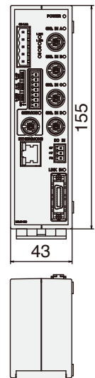
Main unit MG41-NC (for CC-Link, Ethernet)
